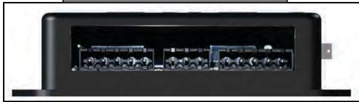
Fig. 3 - Controller Connections
