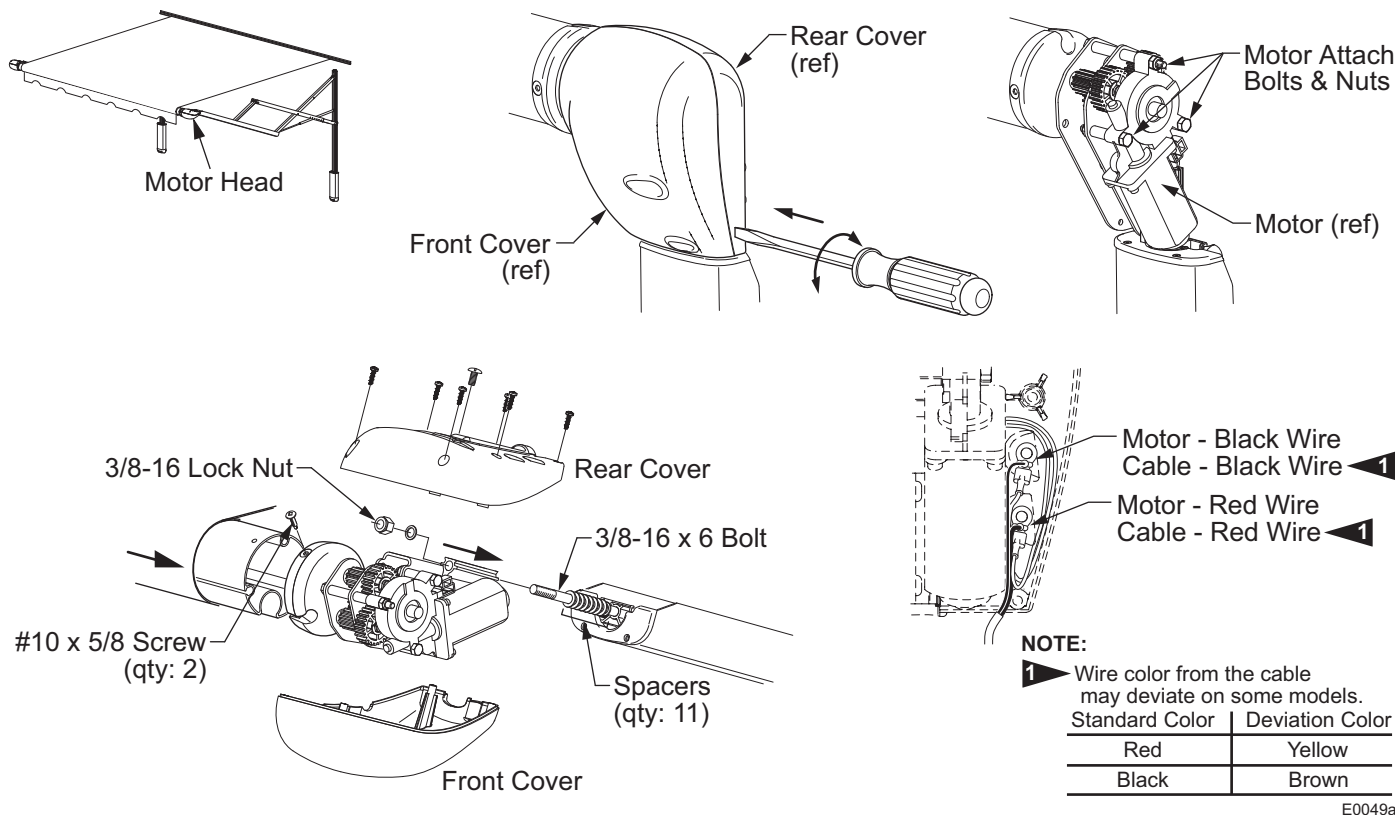
Figure 7. Motor Replacement - Awning Closed.
