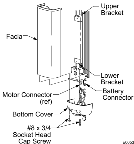
Figure 10. Battery Replacement.
