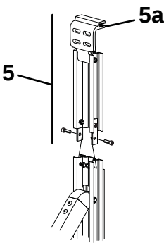
Detail B After Market Top Bracket
