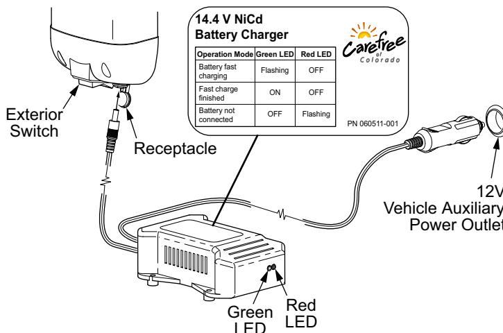
Figure 11. Charging the Battery.
