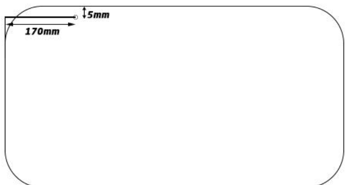
Figure 1 LED Power Loom Access Hole Location (Not to scale)
